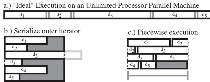
Fig. 1. Approaches to Executing Potential Parallelism
