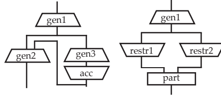
Fig. 9. Pathological Program Configurations
