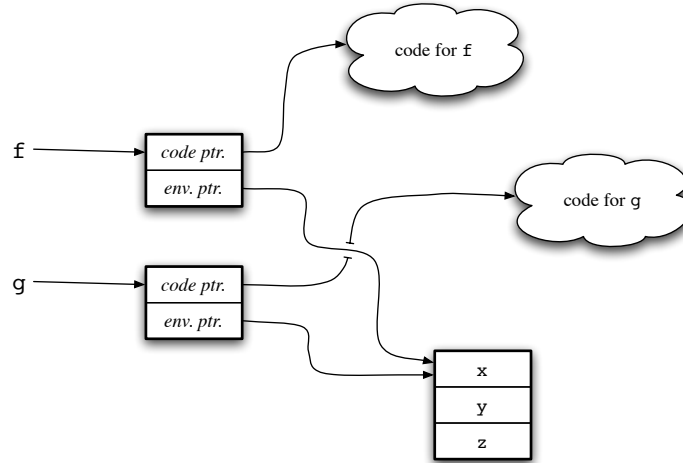
Figure 1: Representation of mutually-recursive functions
